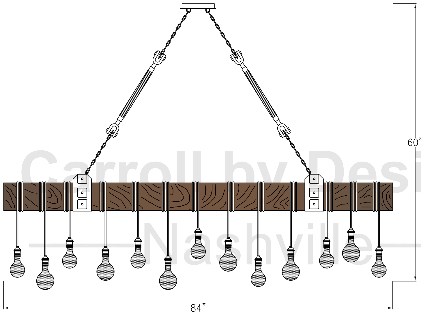
Front View
