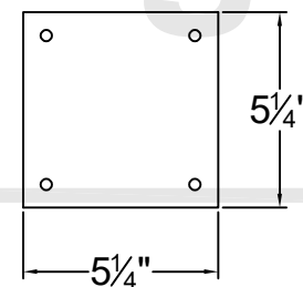
Ceiling Mount
