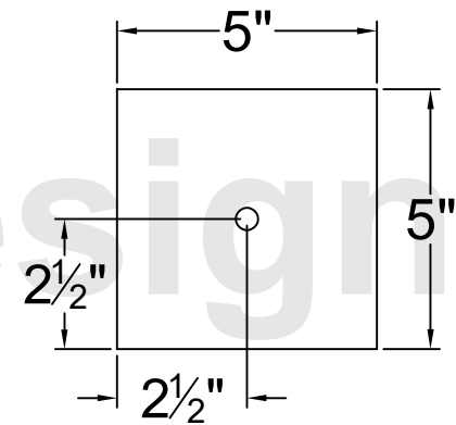
Backplate
