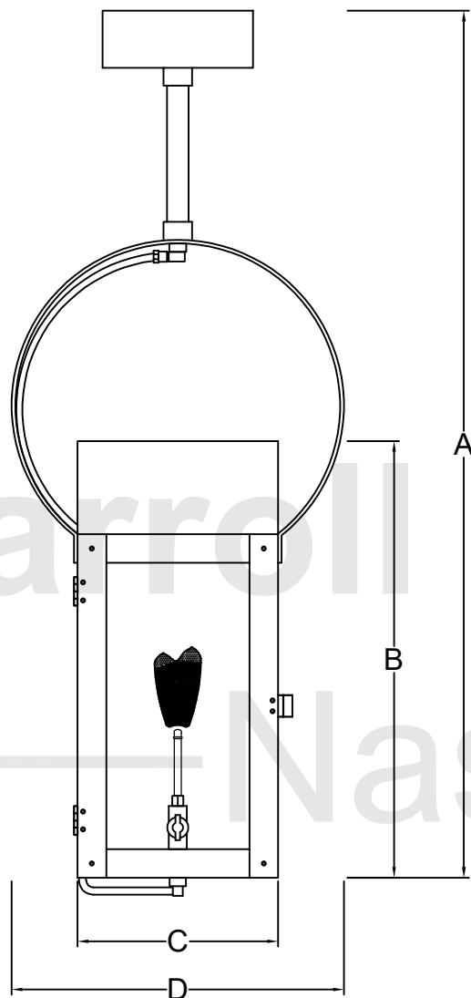
Front View
